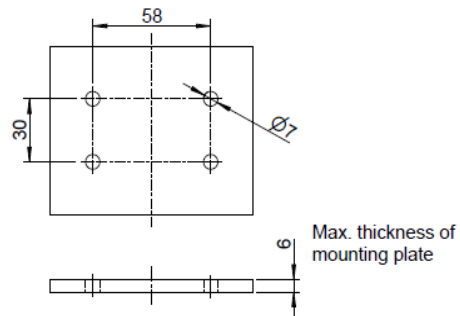
Mounting template
