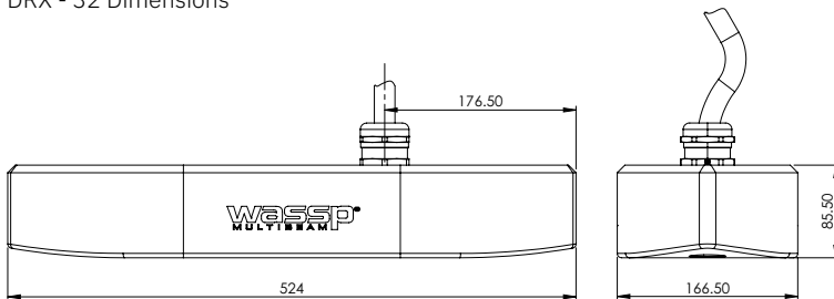
Wideband Fairing Transducer – Dimensions
